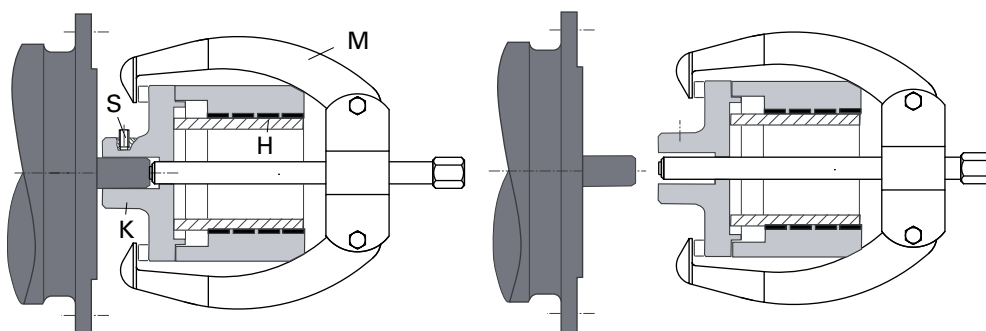
Fig. 3: Extracting the coupling half
