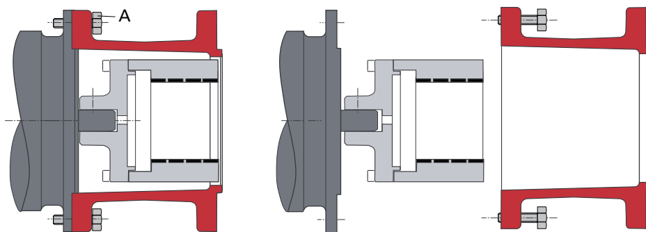
Fig. 2: Dismantling lantern
