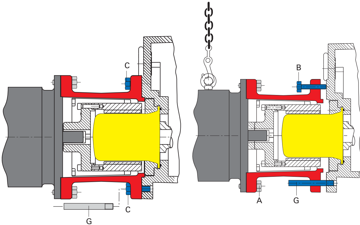
Fig. 1: Dismantling motor and lantern
