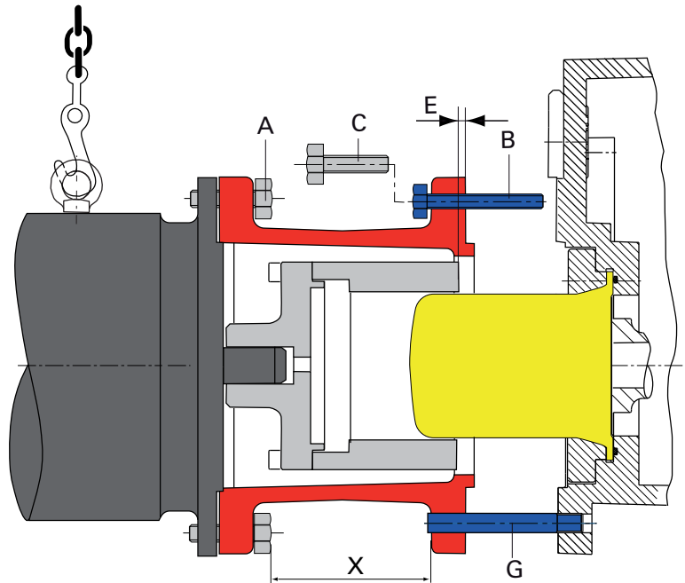
Fig. 4: Assembling drive motor with pre-assembled lantern
